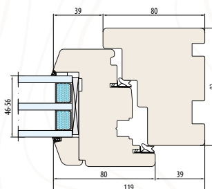
SYSTEM NATURO 92 Innere Fensterbankfräsung
